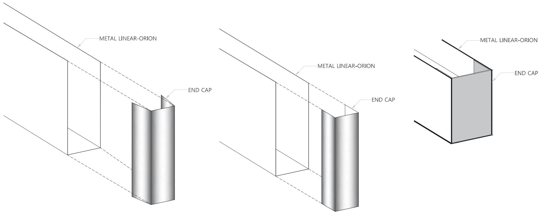
ORION METAL LINEAR END CAP DETAIL
